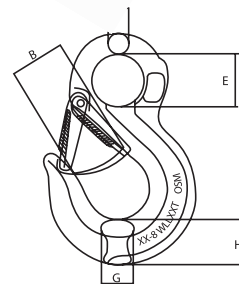
Alloy Eye Sling Hook Grade 80 c/w Latch Type: HEL
