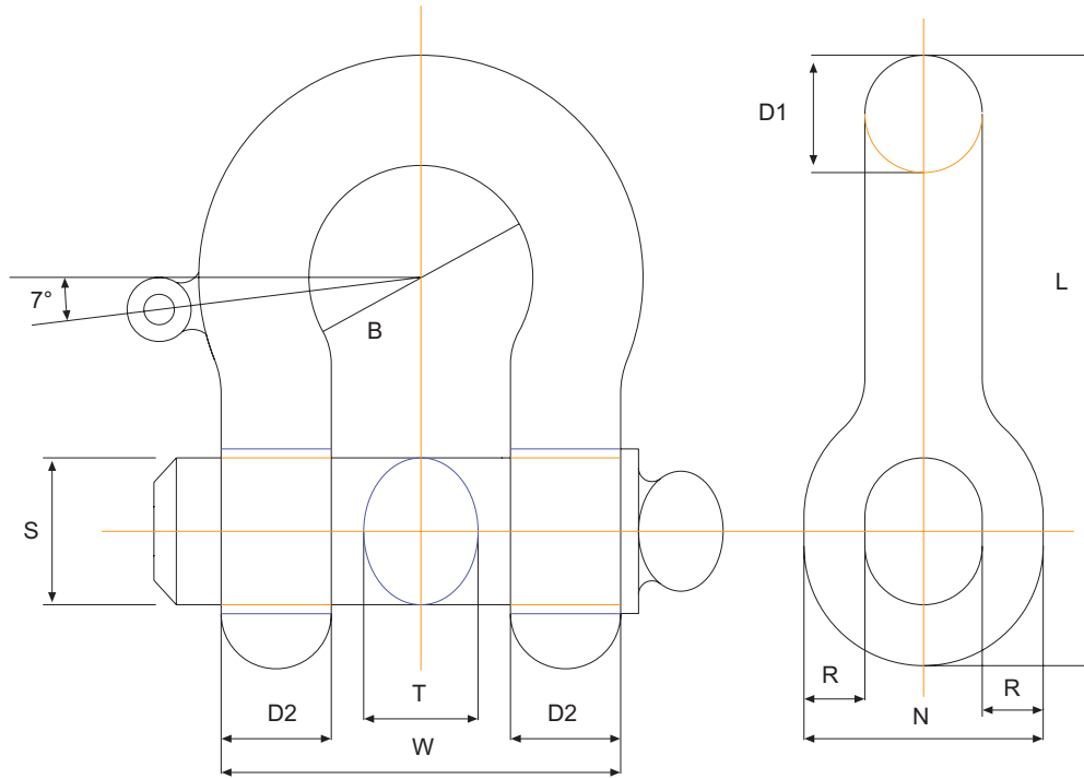
Buoy Shackles (B Type)
